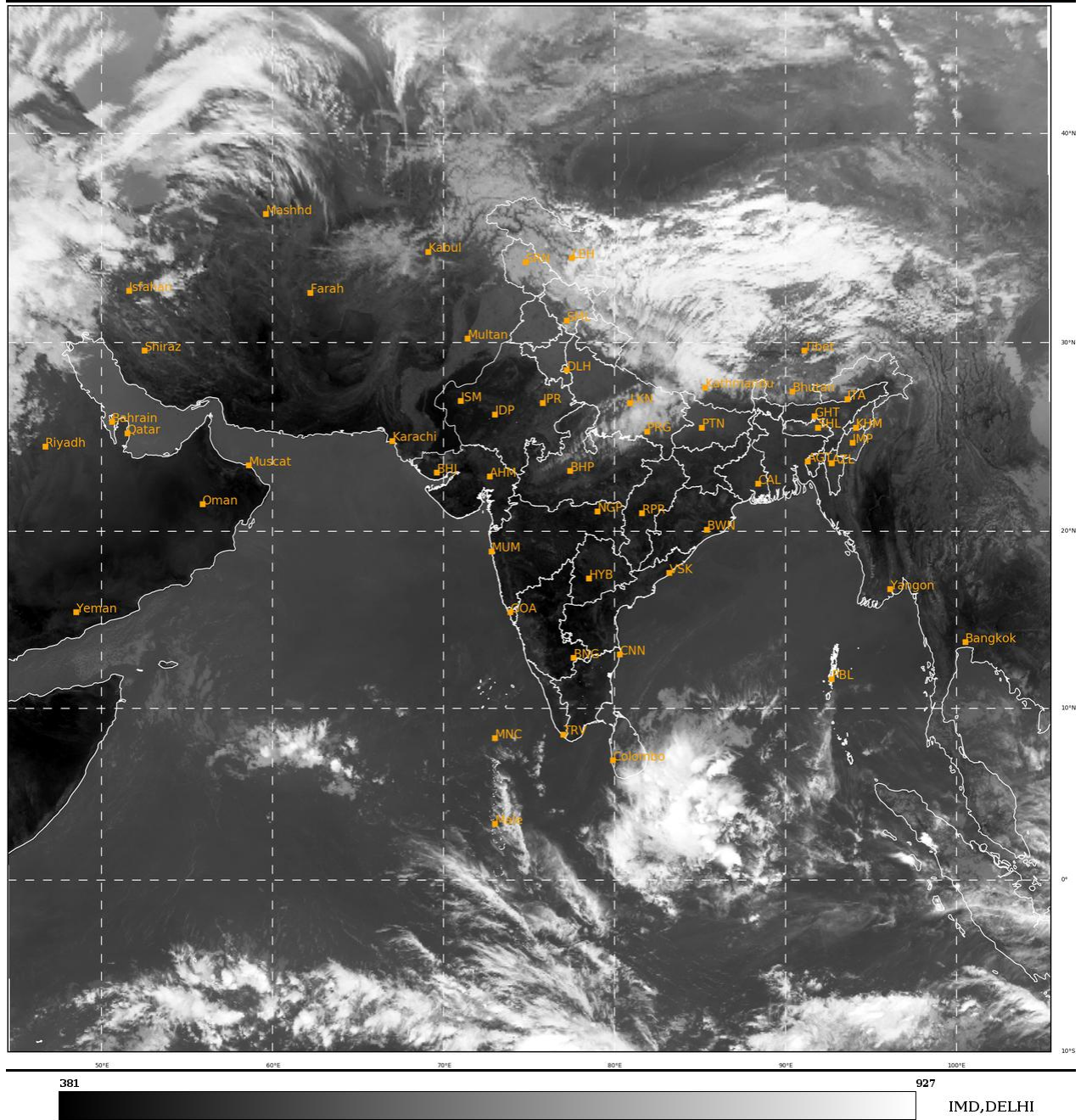
Figure: 1. Latest available satellite picture as on 05 February 2021 at 1357 Hrs (IST). (Source: IMD).
